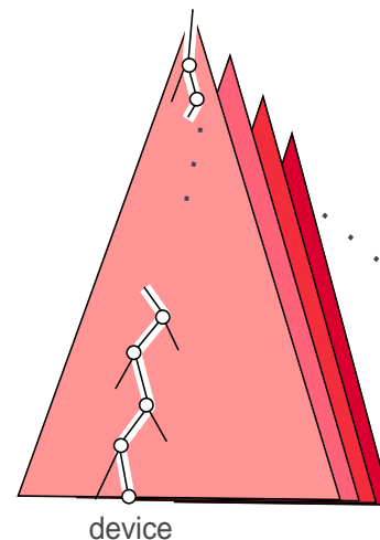
Figure 3-2 Subset-difference Tree
